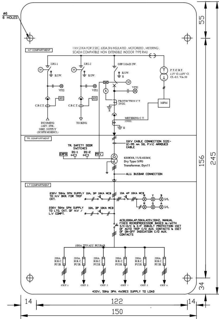
Single Line Deigram (SLD)
